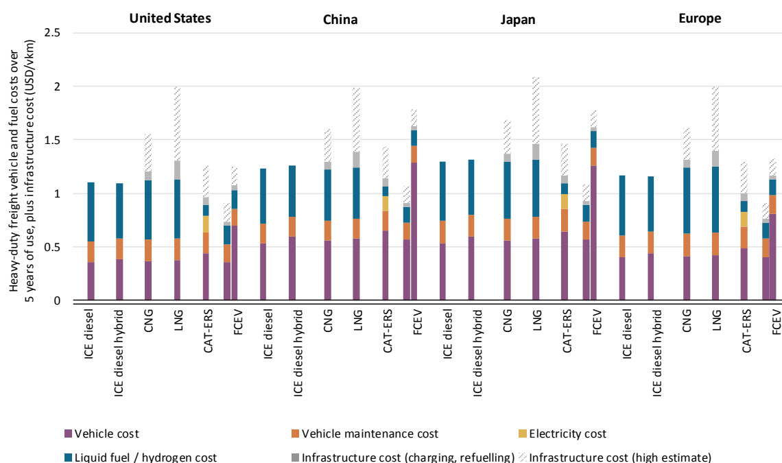
Figure 38 • Heavy-duty freight vehicle and fuel costs over five years of usage in 2050 in the Modern Truck Scenario, including infrastructure costs (with high and low infrastructure utilisation assumptions)
