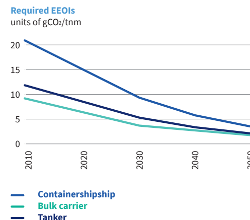
Figure 1 Demand and required aggregate Energy Efficiency Operation Indicator (EEOI) consistent with shipping's 2.33% share of total CO 2 and a 2°C stabilisation pathway taken from our Low Carbon Pathways 2050 report.
