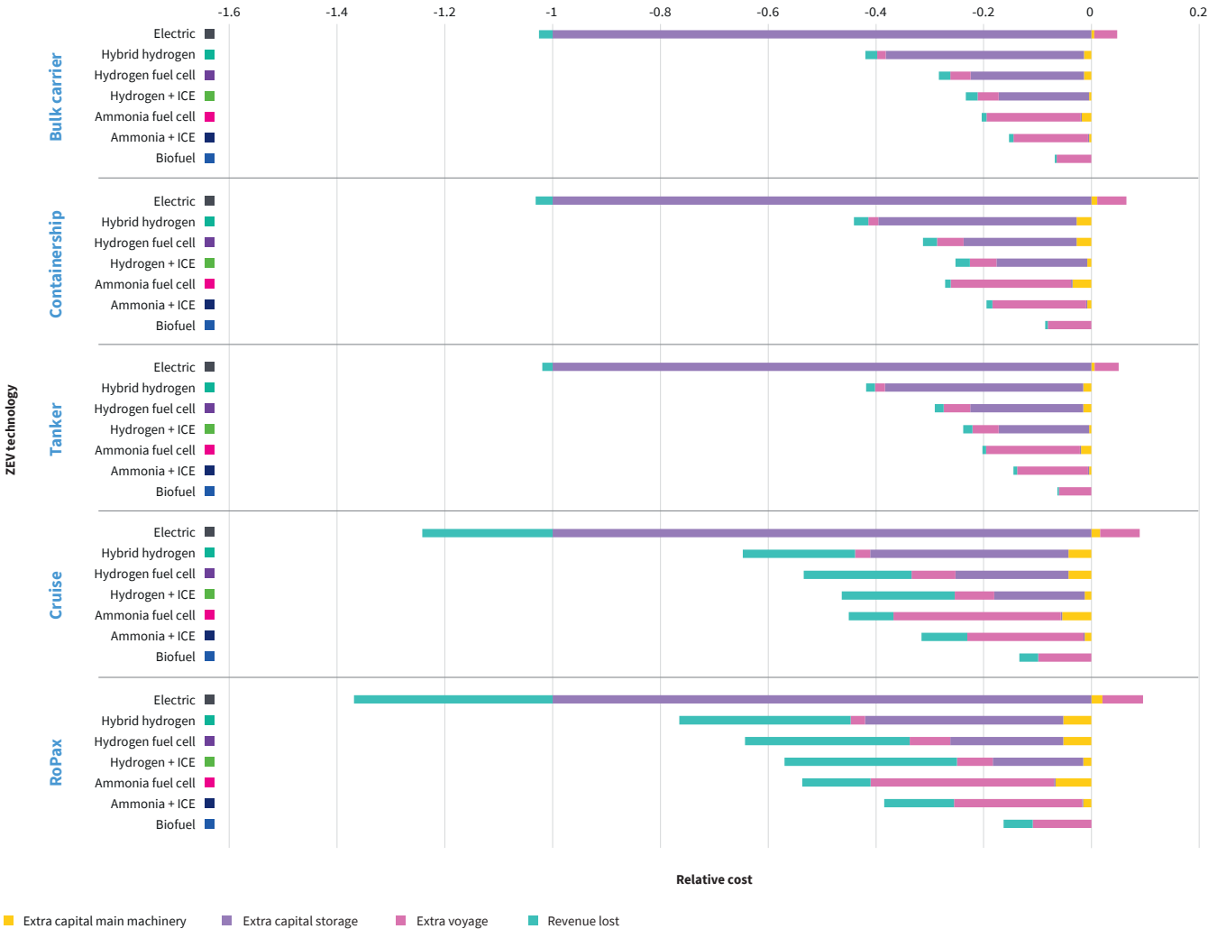
Figure 8 Relative cost implications of ZEV technologies for all ship types under the Green Ammonia scenario against the HFO reference ship
