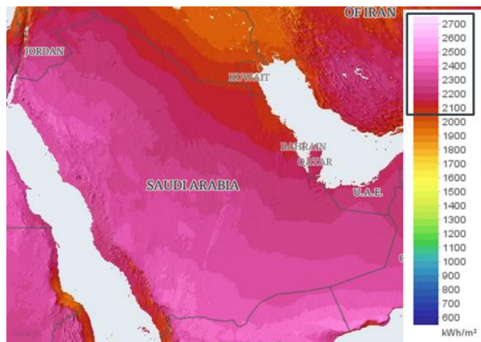
Figure 58. Heat map of solar power, Saudi Arabia
