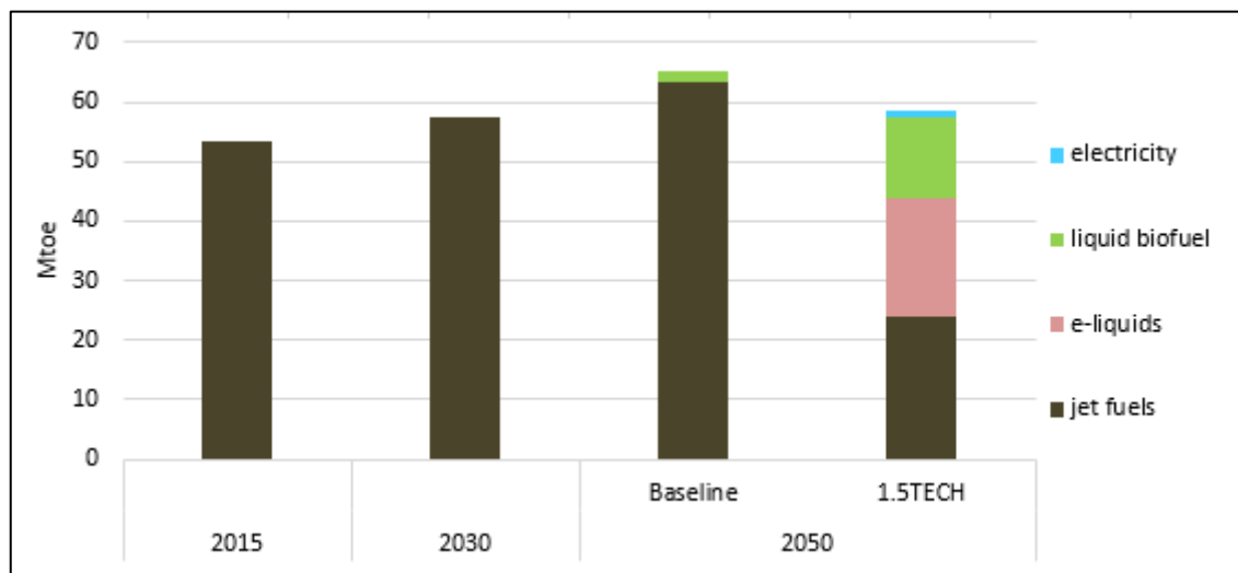
Figure 6-11. Market development: EU aviation, by fuel type and scenario Source: adapted from (EC, 2018c)
