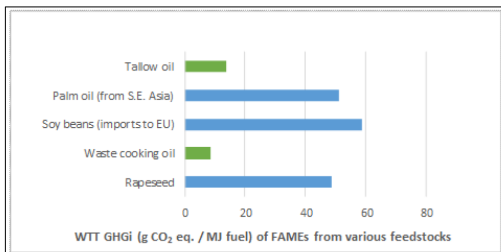
Figure 4-24. Well-to-tank production emissions performances for selected biodiesel pathways
