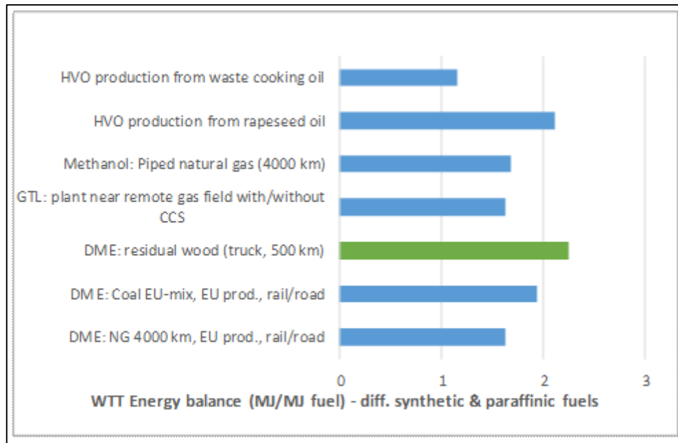
Figure 4-29. Well-to-tank production energy performances for various synthetic and paraffinic fuels Source: JEC-WTT, 2019
