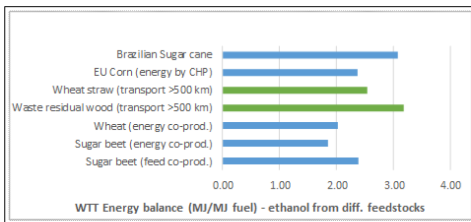
Figure 4-25. Well-to-tank production energy performances for selected bioethanol pathways
