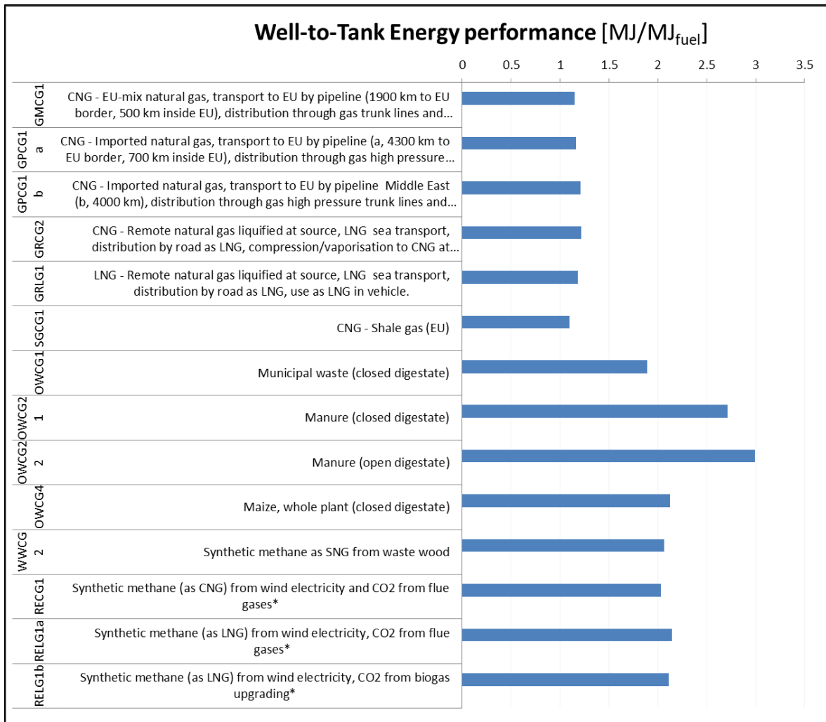
Figure 4-18. Well-to-tank production energy performances for selected pathways (* These are e-fuels; more details on e-fuels can be found in section 4.4.3, p. 63)
