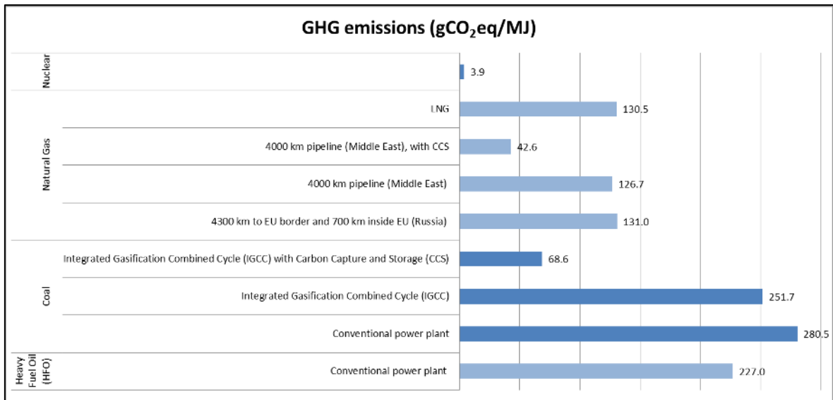
Figure 4-7. Fossil primary energy sources and nuclear fission to electricity: GHG emissions (gCO 2 eq/MJ)
