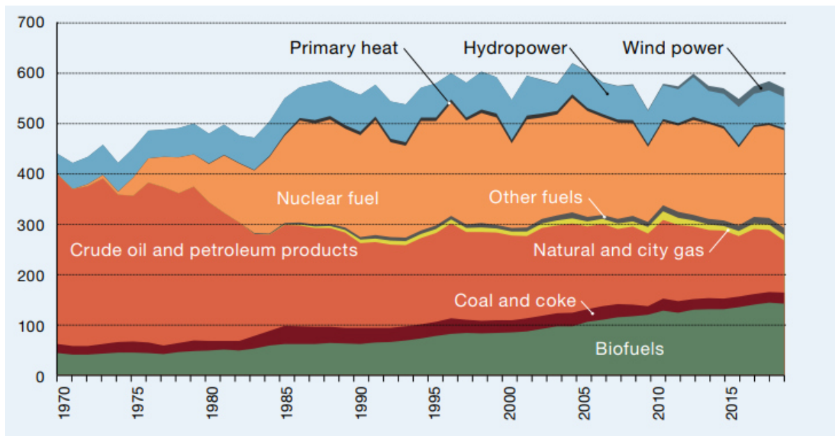
Figure 7: Supply of energy in Sweden 1970-2018, TWh, Sources: Swedish Energy Agency and Statistics Sweden
