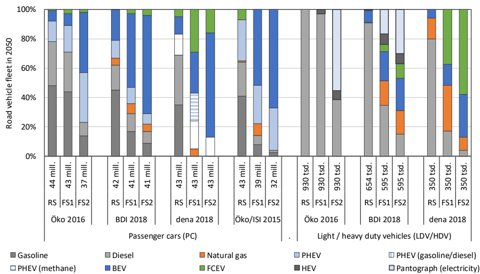
Figure 16: Vehicle fleet scenario Germany in 2050 (DBFZ based on Wietschel et al) 43
