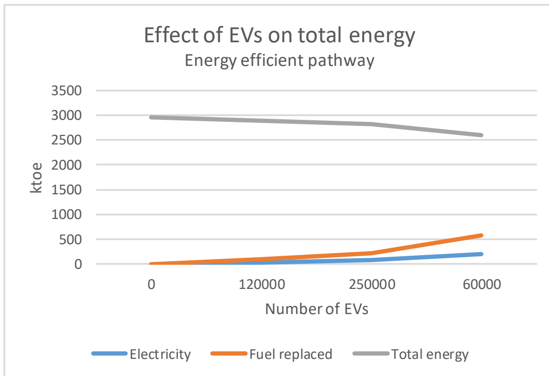
Figure 4. The effects of electrification on total energy demand and fuel replaced, calculated for the energy efficient transport system pathway.
