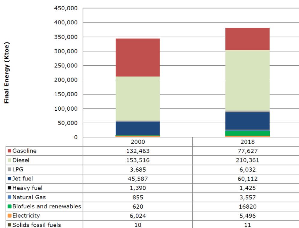
Figure 1: Final energy mix in the transport sector of the EU28 in 2000 compared to 2018 (Source: JRC 2020)
