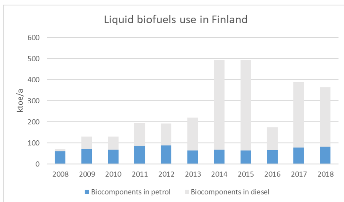
Figure 4: Volumes of liquid biofuels in Finland 1
