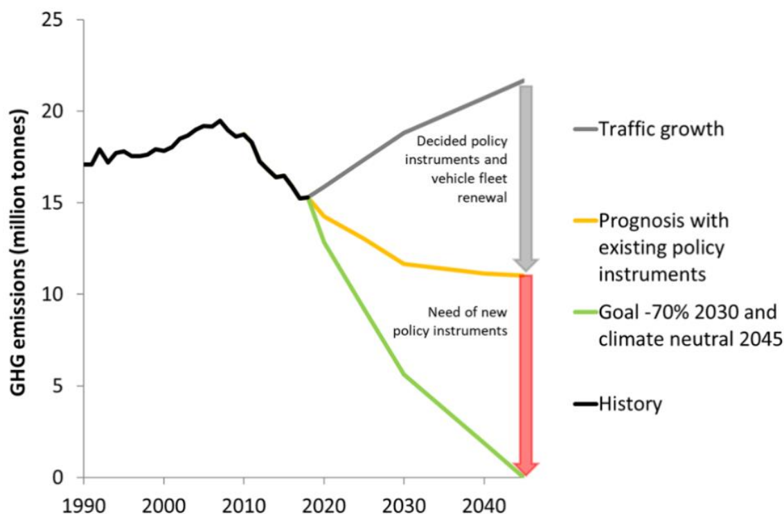
Figure 12: The gap between BAU scenario and the goals for the Swedish transport sector. Source: Swedish Transport Administration
