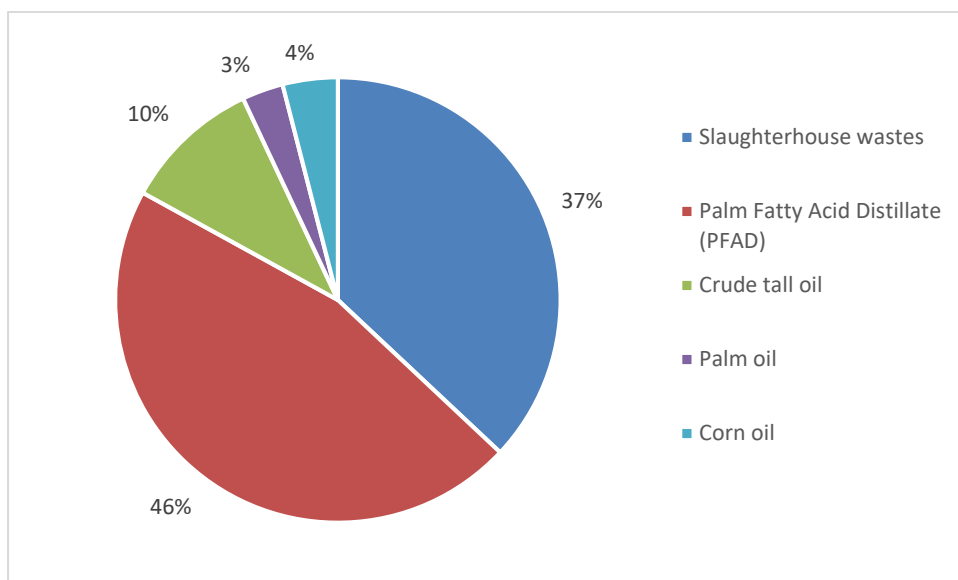
Figure 9: Raw materials for HVO used in Sweden 2018. Source: Swedish Energy Agency
