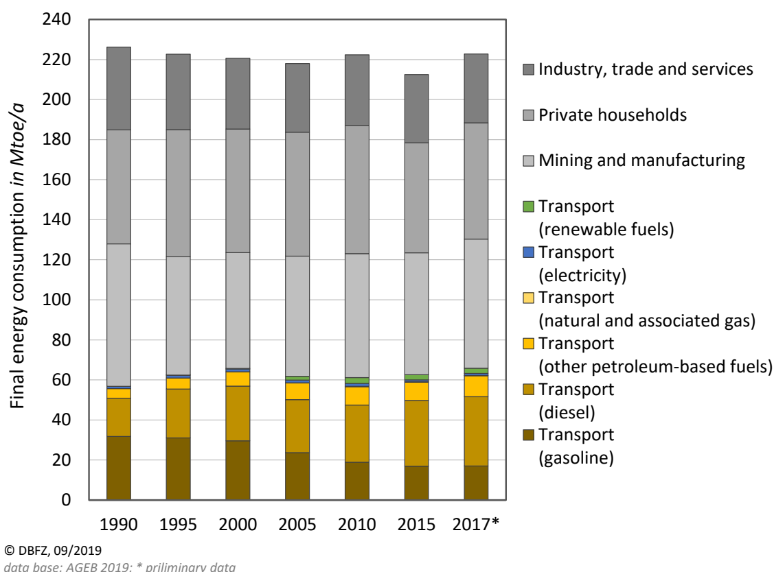
Figure 13: Development of the energy demand of different sectors (DBFZ based on AGEB 2018) 31
