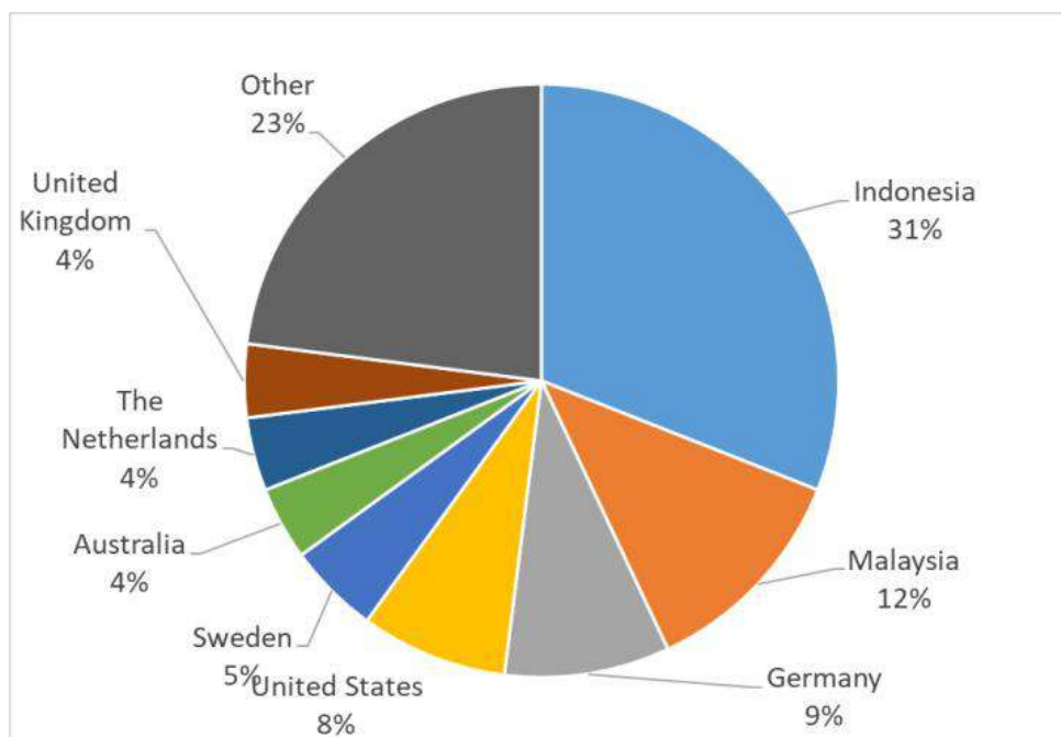
Figure 10: Country of feedstock origin for HVO consumed in Sweden in 2017
