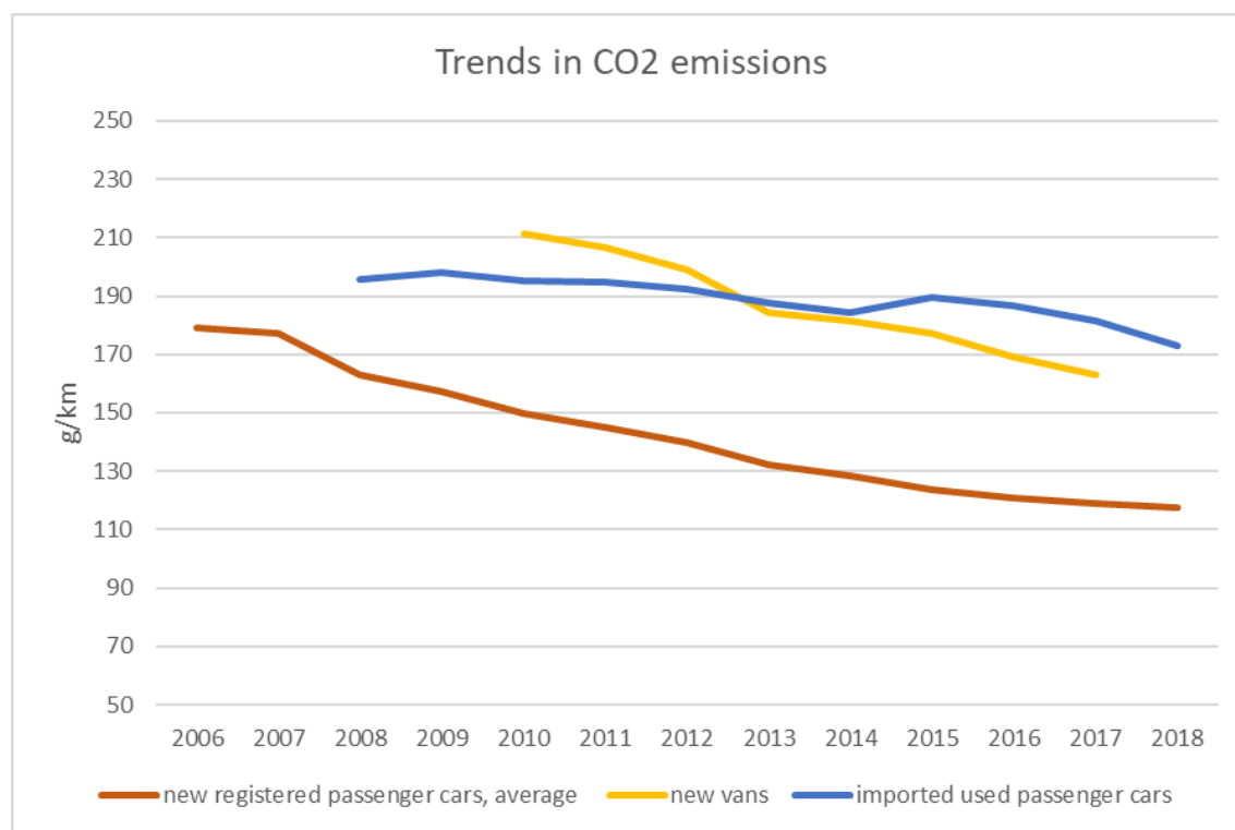
Figure 6: Trends in CO 2 emissions of new passenger cars and vans and used imported passenger cars 8 .
