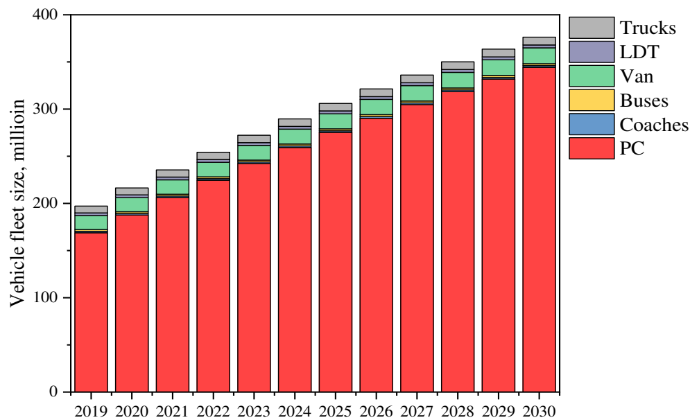
Figure 31: The prediction of future vehicle stock in China (high scenario)
