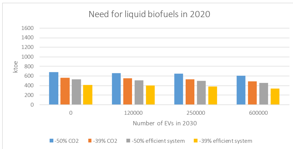
Figure 6. The need for liquid biofuels in 2020.
