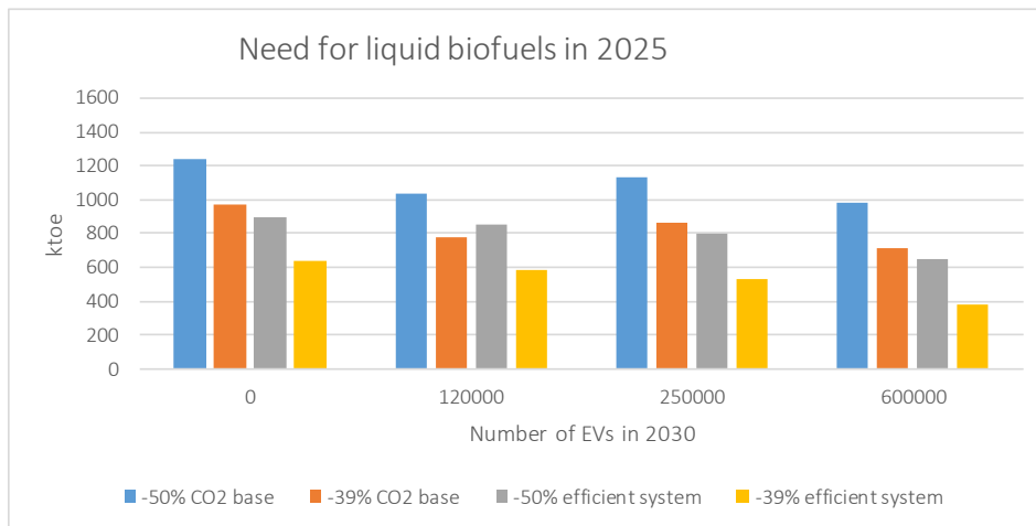
Figure 7. The need for liquid biofuels in 2025.
