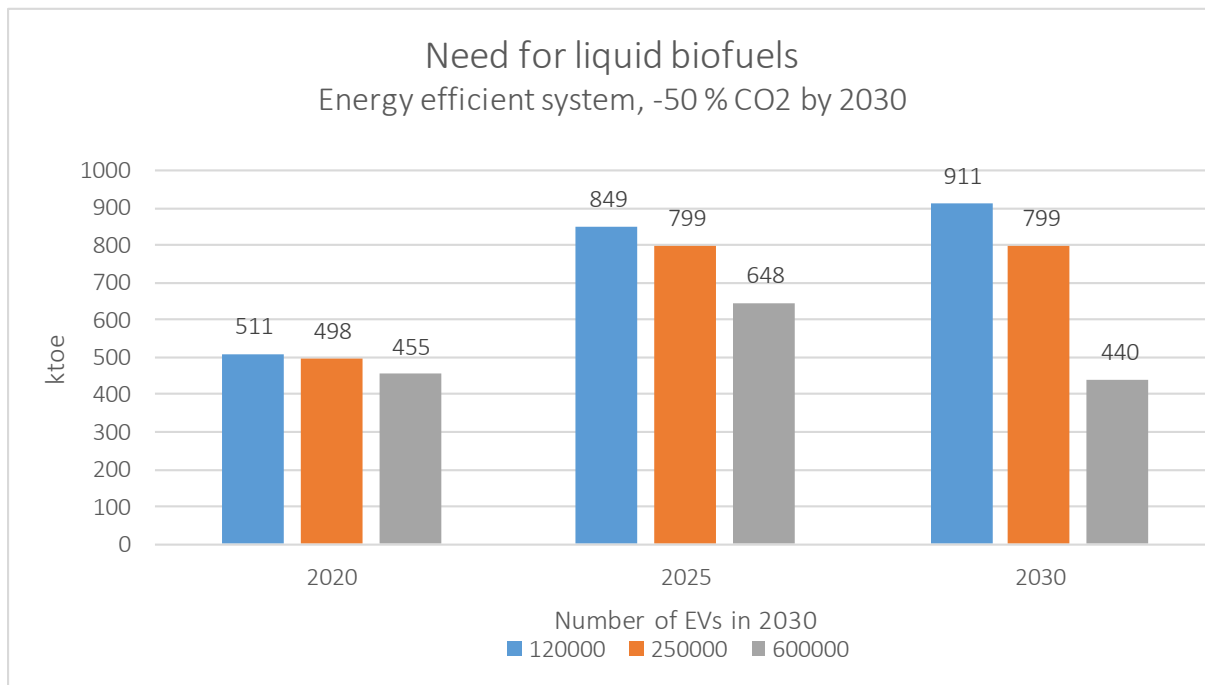
Figure 9. The need for liquid biofuels in an energy efficient transport system.
