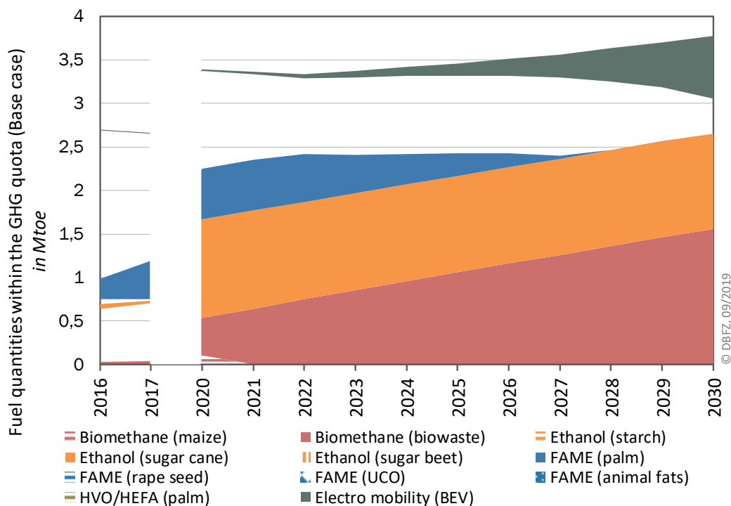
Figure 18: Base case scenario – fuel quantities within the GHG quota until 2030
