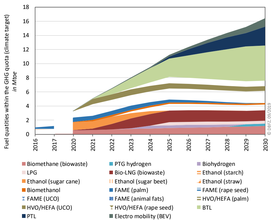
Figure 19: Climate scenario – fuel quantities within the GHG quota until 2030
