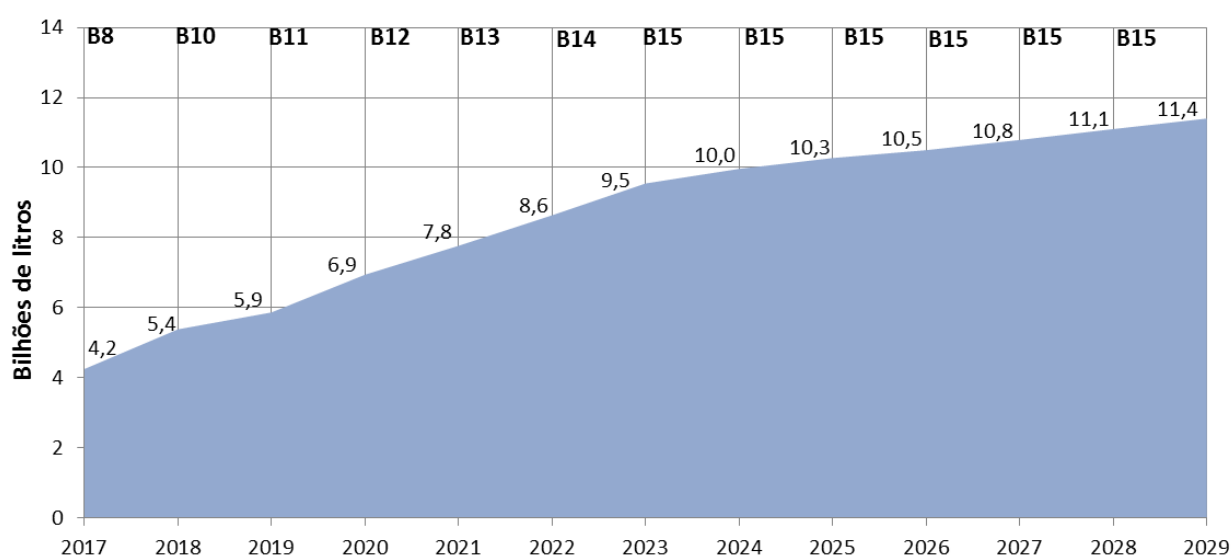
Figure 28: Projected biodiesel production to 2029
