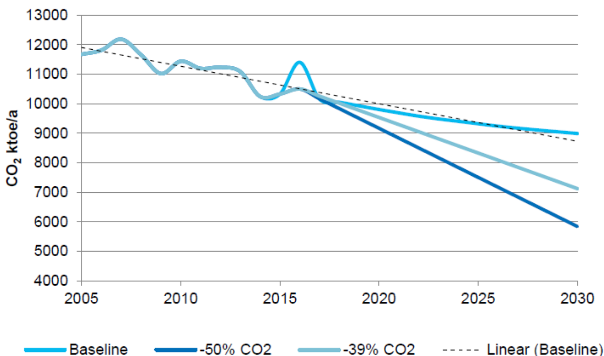
Figure 5: Road transport CO 2 inventory from 2005 (reference year) to 2030 (target year) and the trajectories needed to reach emission reductions of -39 or -50% by 2030 4 .
