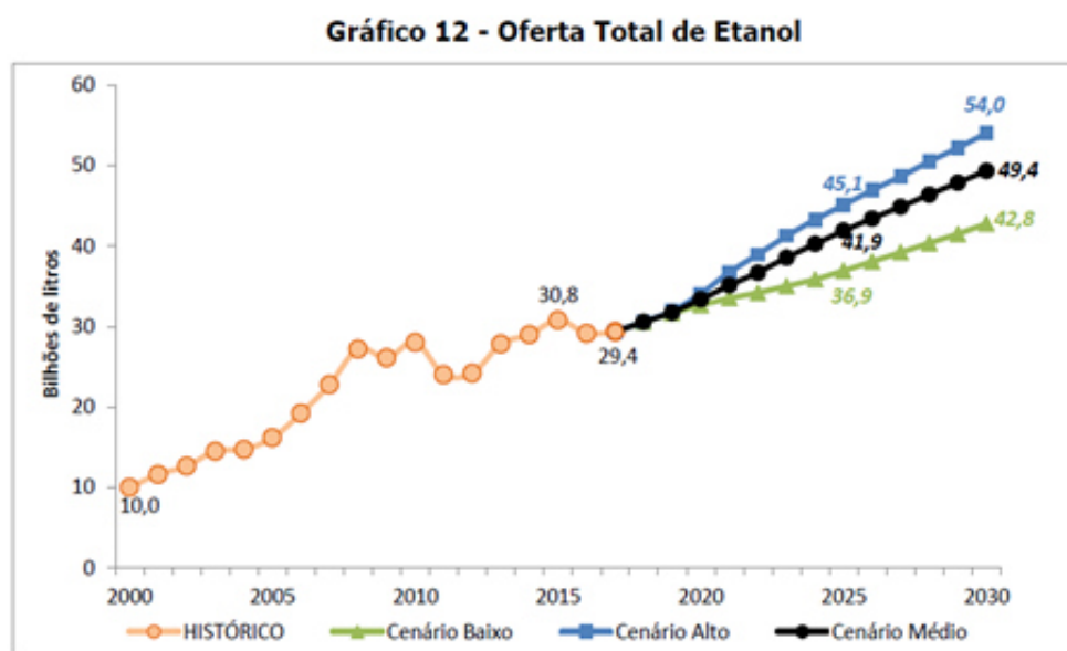
Figure 27: Historic and projected ethanol supply for three scenarios 102
