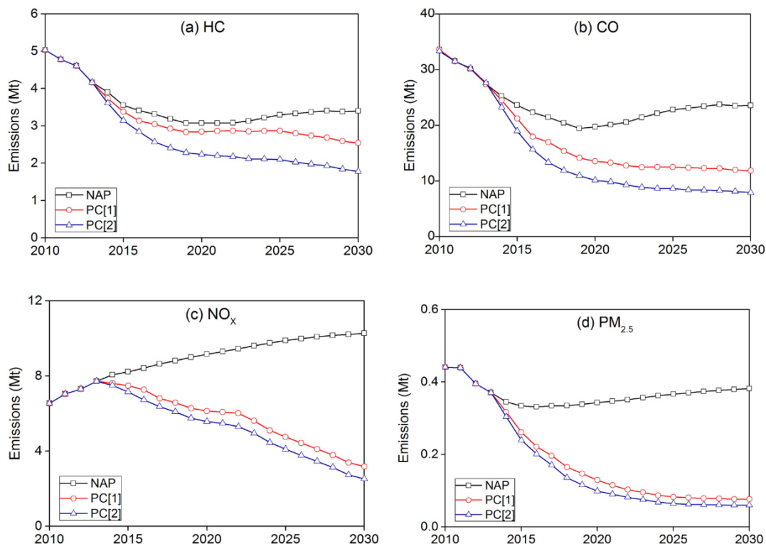
Figure 32: The future emission trends for on-road vehicles in China under three designed policy cases (note: emissions of gasoline-powered motorcycles included)
