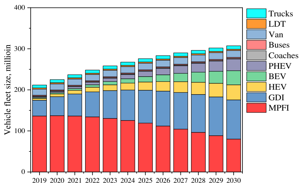
Figure 30: The prediction of future vehicle stock in China (low scenario)
