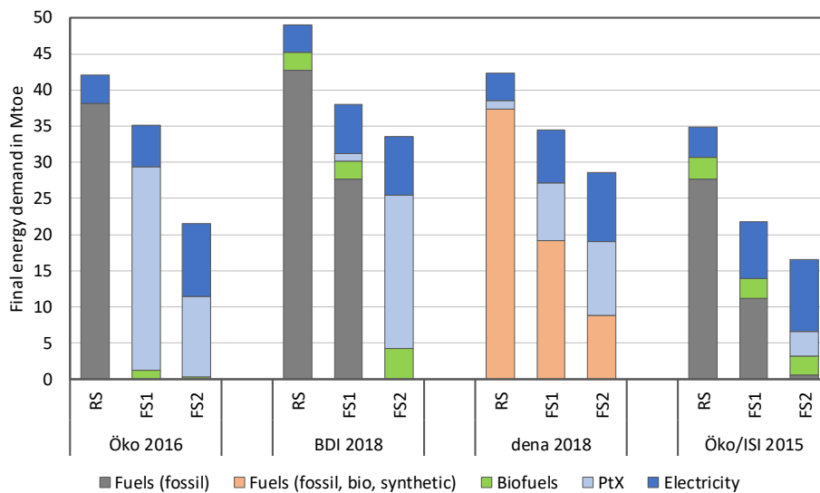
Figure 17: Final energy demand of German transport sector in 2050 (DBFZ based on Wietschel et al) 43
