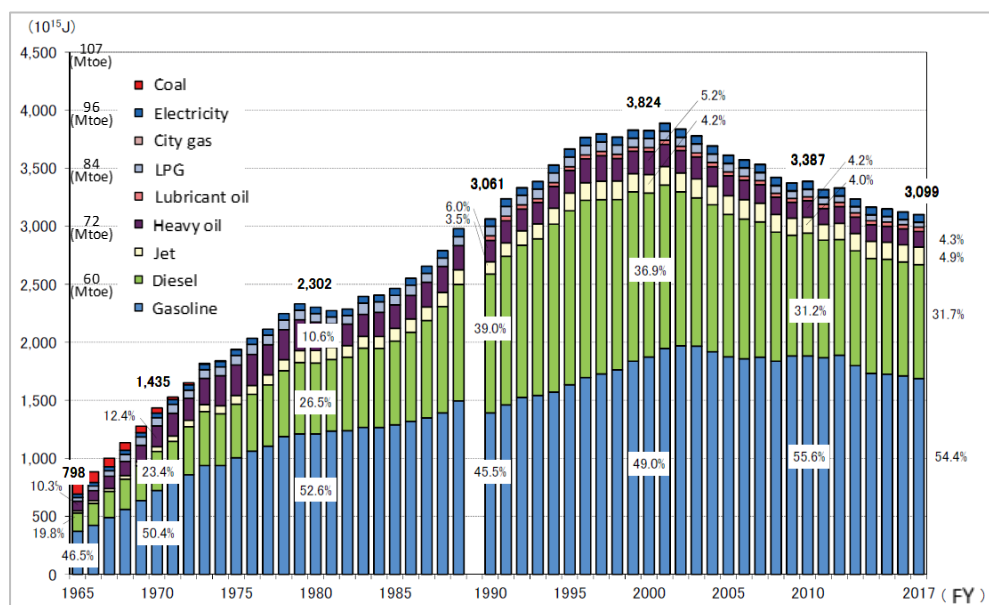
Figure 34: Trends in energy consumption in the transport sector 114 .
