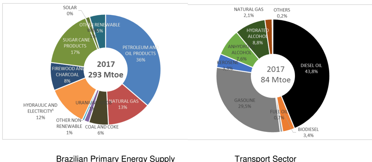
Figure 25: The Brazilian primary energy supply and Final consumption energy for transports in 2017
