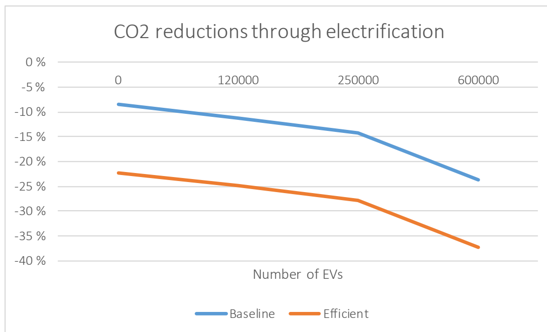
Figure 5. Levels of CO 2 reductions (relative to 2005) that can be reached with electrification only.
