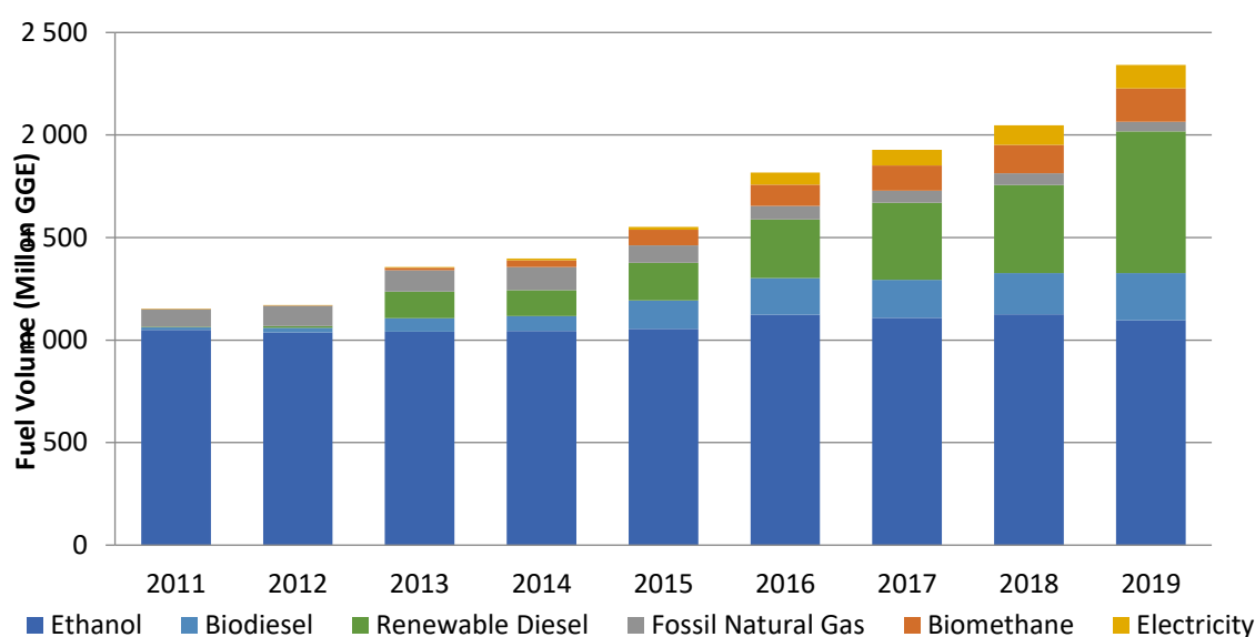
Figure 23: Renewable fuel growth resulting from California's LCFS (2011-2019)
