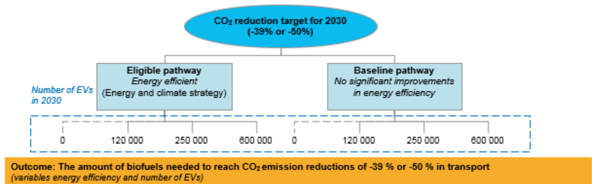
Figure 2. Evaluated scenarios, main variables are CO 2 reduction target, energy efficiency and number of electric vehicles.
