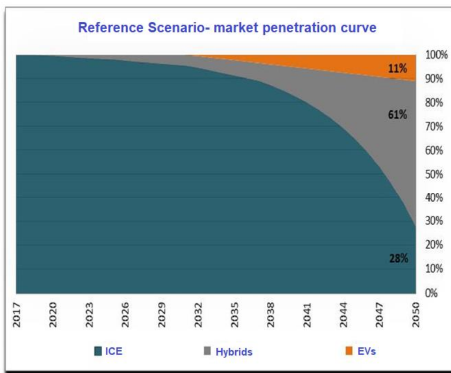
Figure 29: Market penetration of hybrid and EV light duty vehicles on the Brazilian market 104
