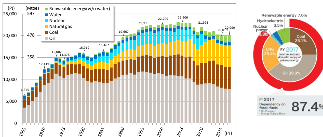
Figure 33: Trends in composition of primary energy supply 113 .
