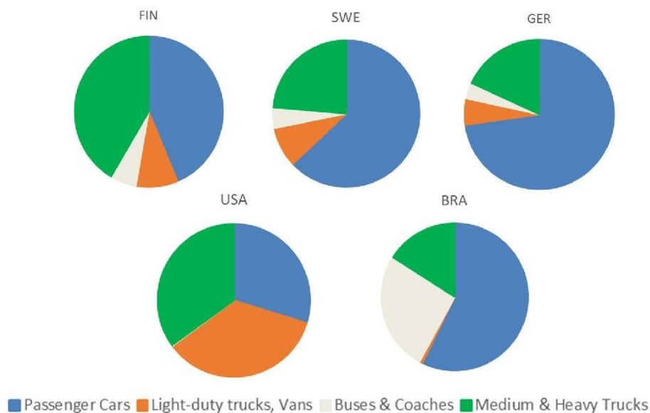
Figure 5: Energy use per vehicle category in Current Policies scenarios – 2030.
