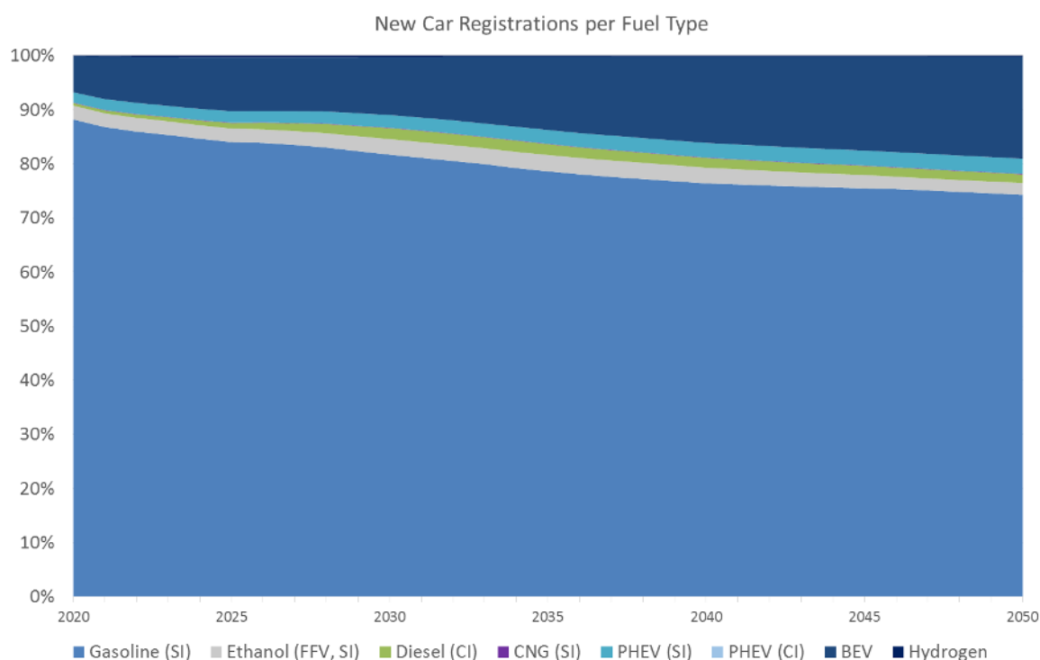
Figure 24: Breakdown of new car sales by powertrain options for the USA in the Current Policies scenario.
