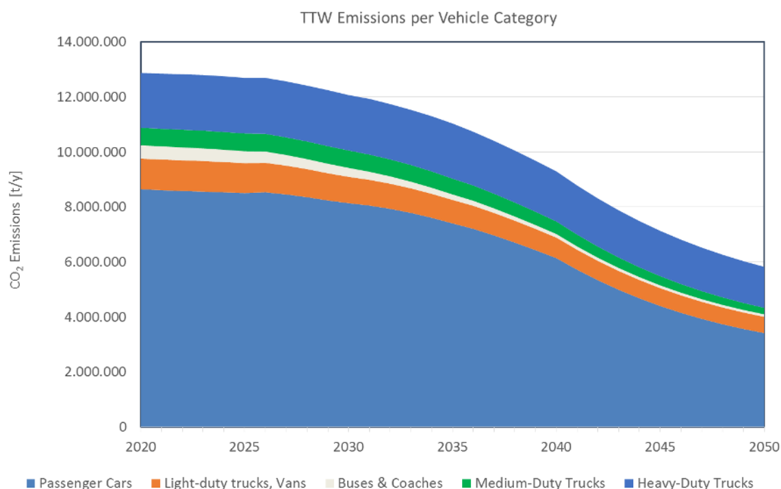
Figure 17: TTW CO 2 emissions in road transport by vehicle category for Sweden in the Current Policies scenario.
