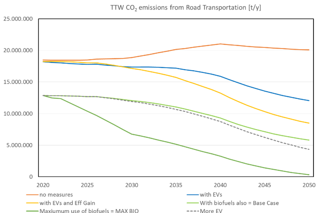
Figure 47: TTW CO 2 emissions evolution by different measures in road transport for Sweden in the MAX BIO scenario.
