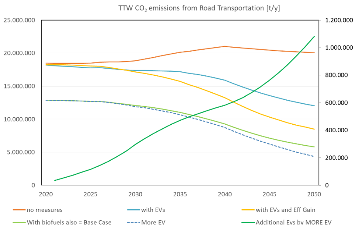
Figure 37: TTW CO 2 emissions in road transport by different measures for Sweden in the MORE EV scenario.
