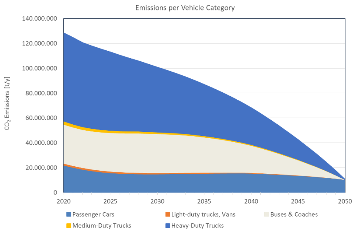
Figure 52: CO 2 Emissions in road transport by vehicle category for Brazil in the MAX BIO scenario.
