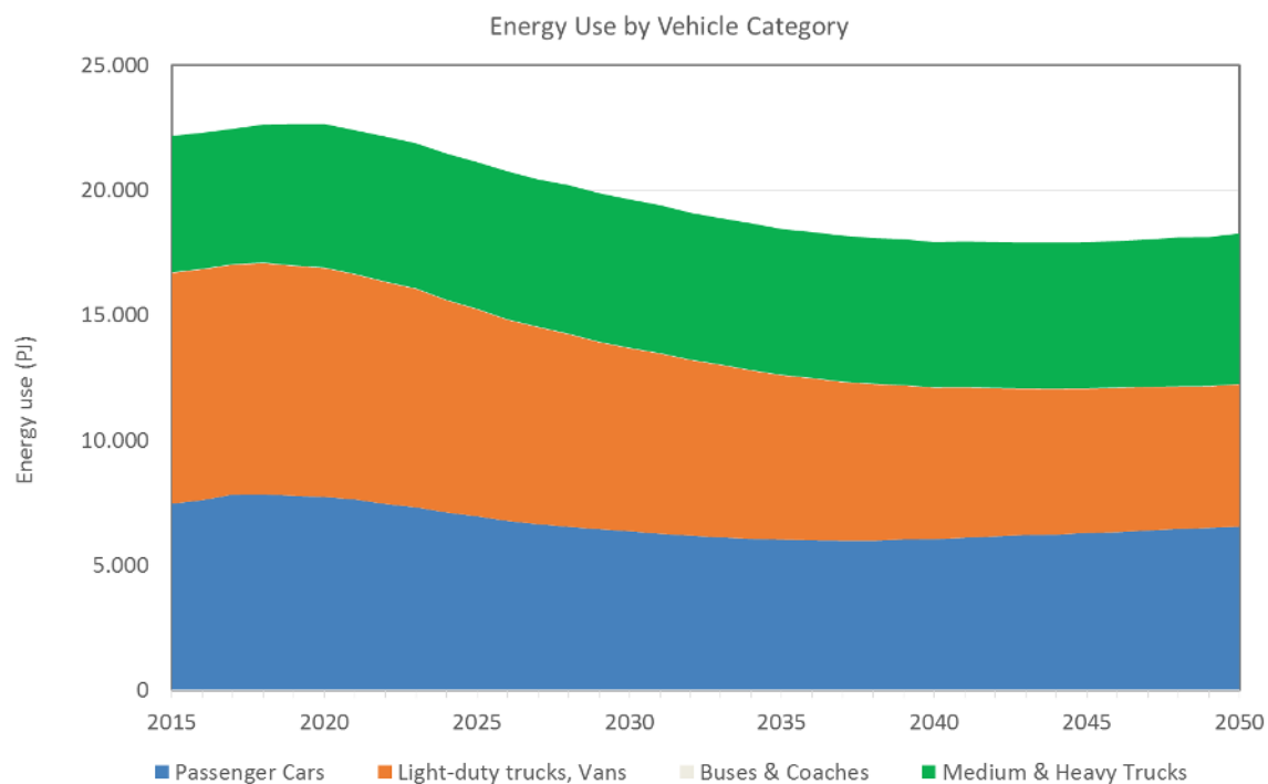
Figure 25: Energy use in road transport by vehicle category for the USA in the Current Policies scenario.
