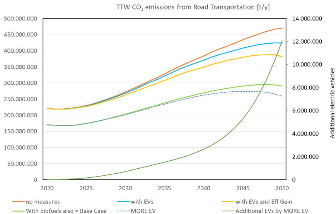
Figure 41: TTW CO 2 emissions in road transport by different measures for Brazil in the MORE EV scenario.
