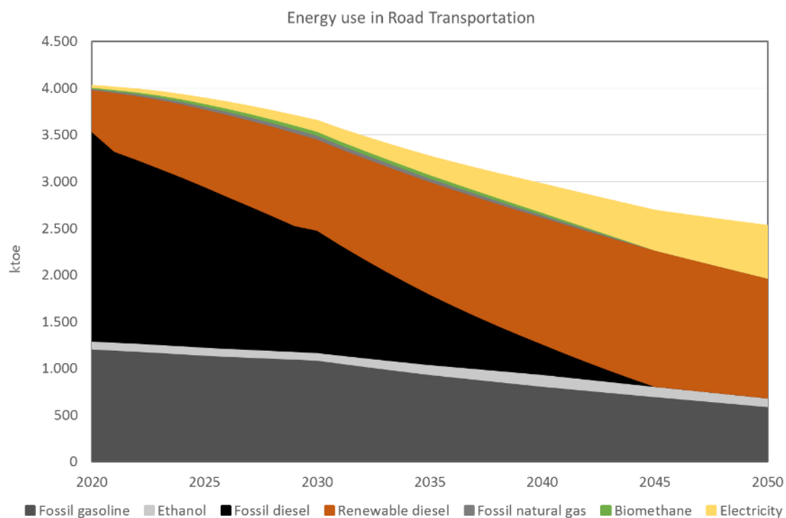
Figure 42: Energy use in road transport by energy carrier for Finland in the MAX BIO scenario.
