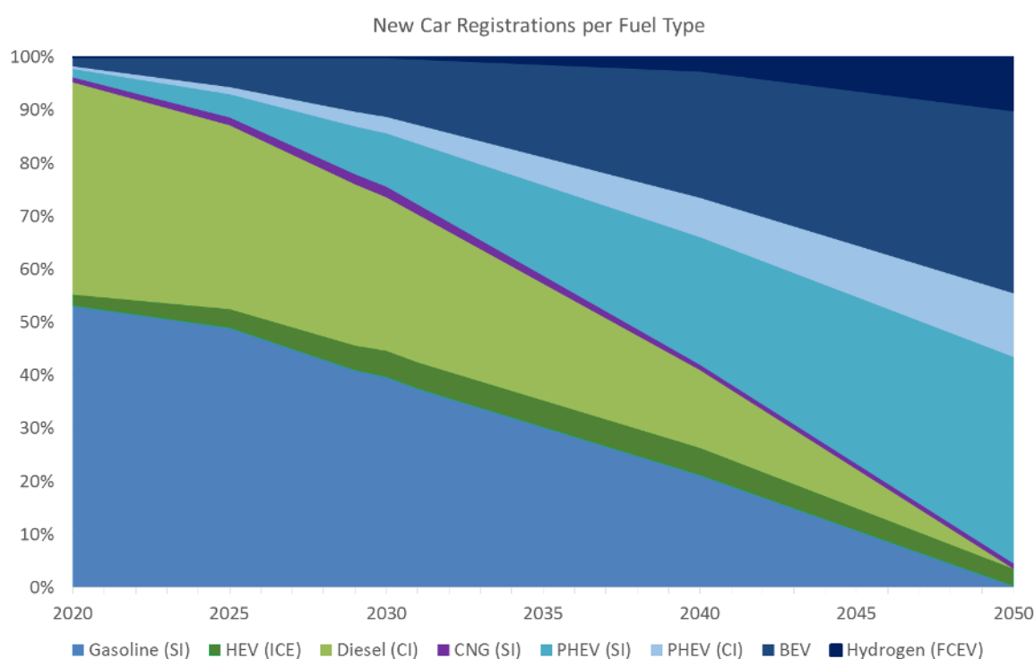
Figure 38: Breakdown of new car sales by powertrain options for Germany in the MORE EV scenario.
