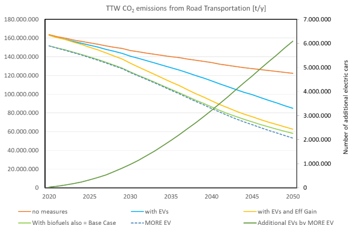
Figure 39: TTW CO 2 emissions in road transport by different measures for Germany in the MORE EV scenario.
