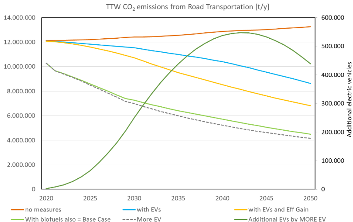
Figure 35: TTW CO 2 emissions in road transport by different measures for Finland in the MORE EV scenario.
