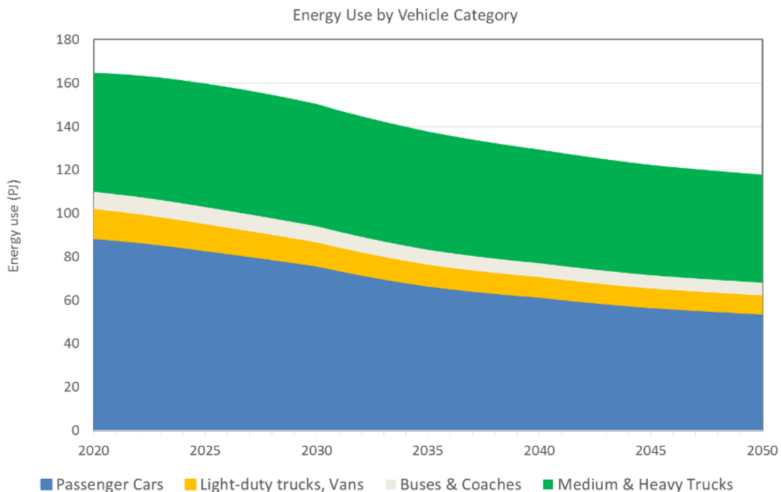
Figure 9: Energy use in road transport by vehicle category for Finland in the Current Policies scenario.
