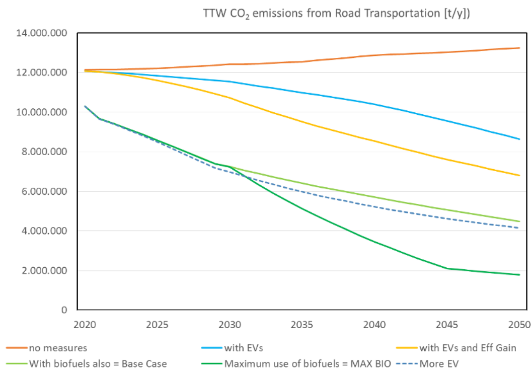
Figure 44: TTW CO 2 emissions evolution by different measures in road transport for Finland in the MAX BIO scenario
