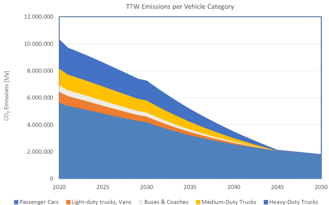
Figure 43: TTW CO 2 Emissions in road transport by vehicle category for Finland in the MAX BIO scenario.
