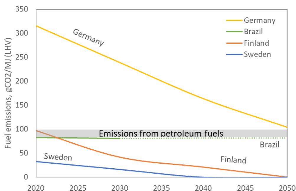
Figure 59: Calculated e-fuel emissions based on national scenarios on the development of average grid emissions. Calculations are made assuming average 40% efficiency from electricity to fuel (LHV).
