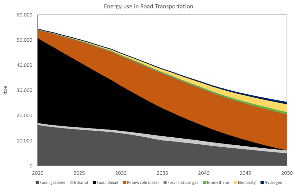
Figure 48: Energy use in road transport by energy carrier for Germany in the MAX BIO scenario.
