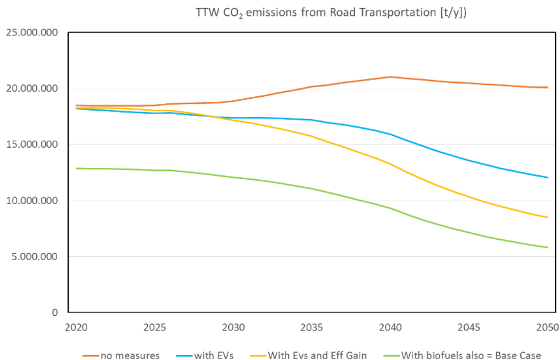
Figure 13: TTW CO 2 emissions in road transport by different measures for Sweden in the Current Policies scenario.
