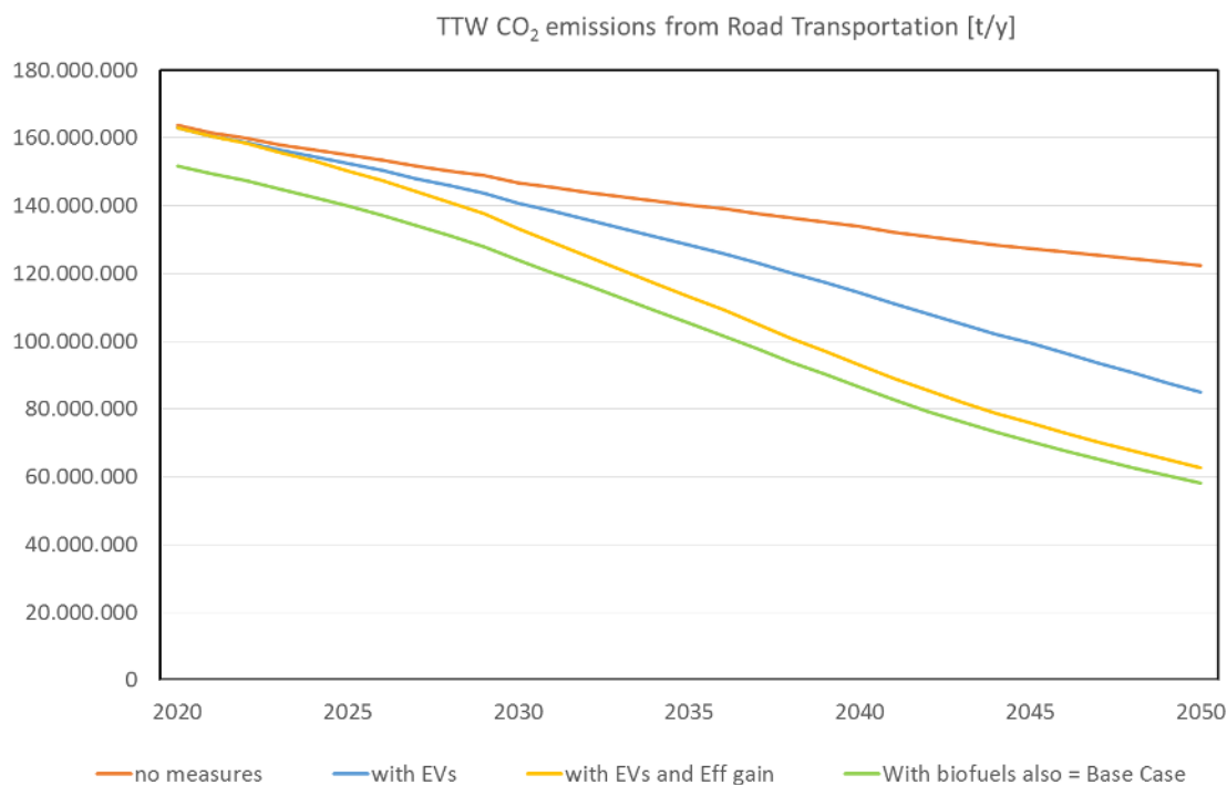
Figure 18: TTW CO 2 emissions in road transport by different measures for Germany in the Current Policies scenario.
